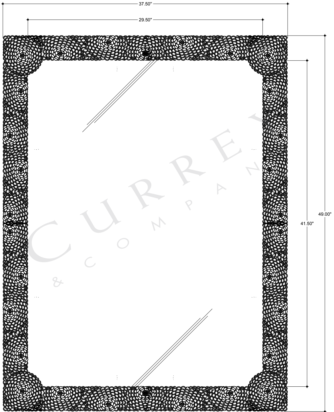
FRONT VIEW
