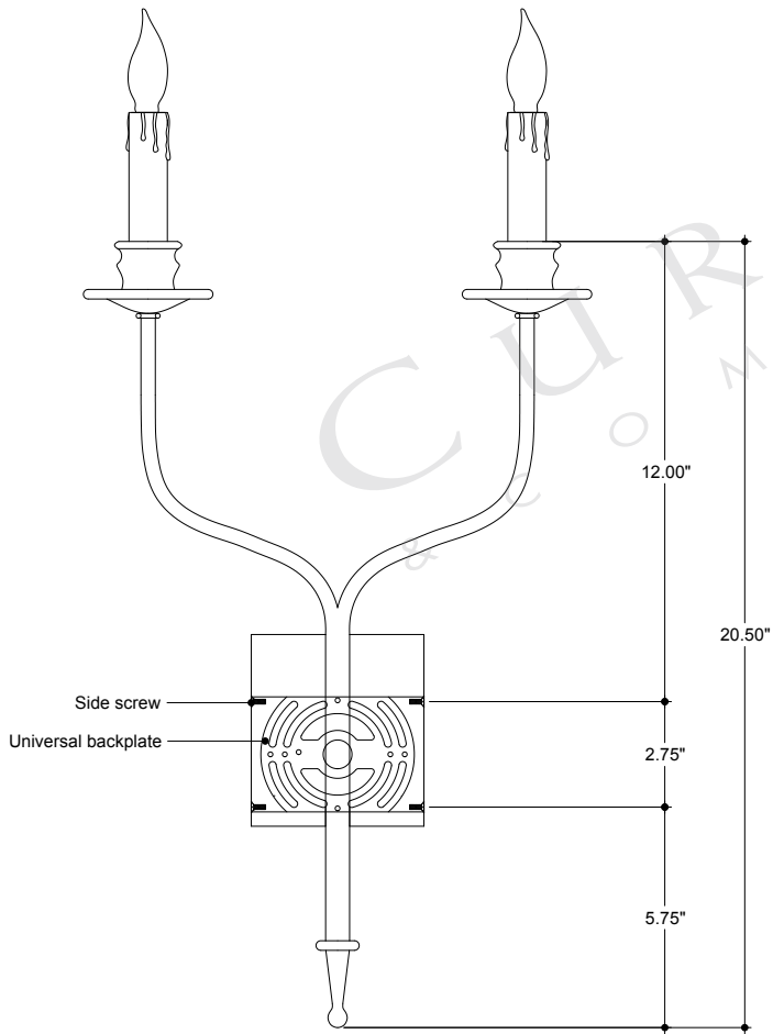
FRONT VIEW
