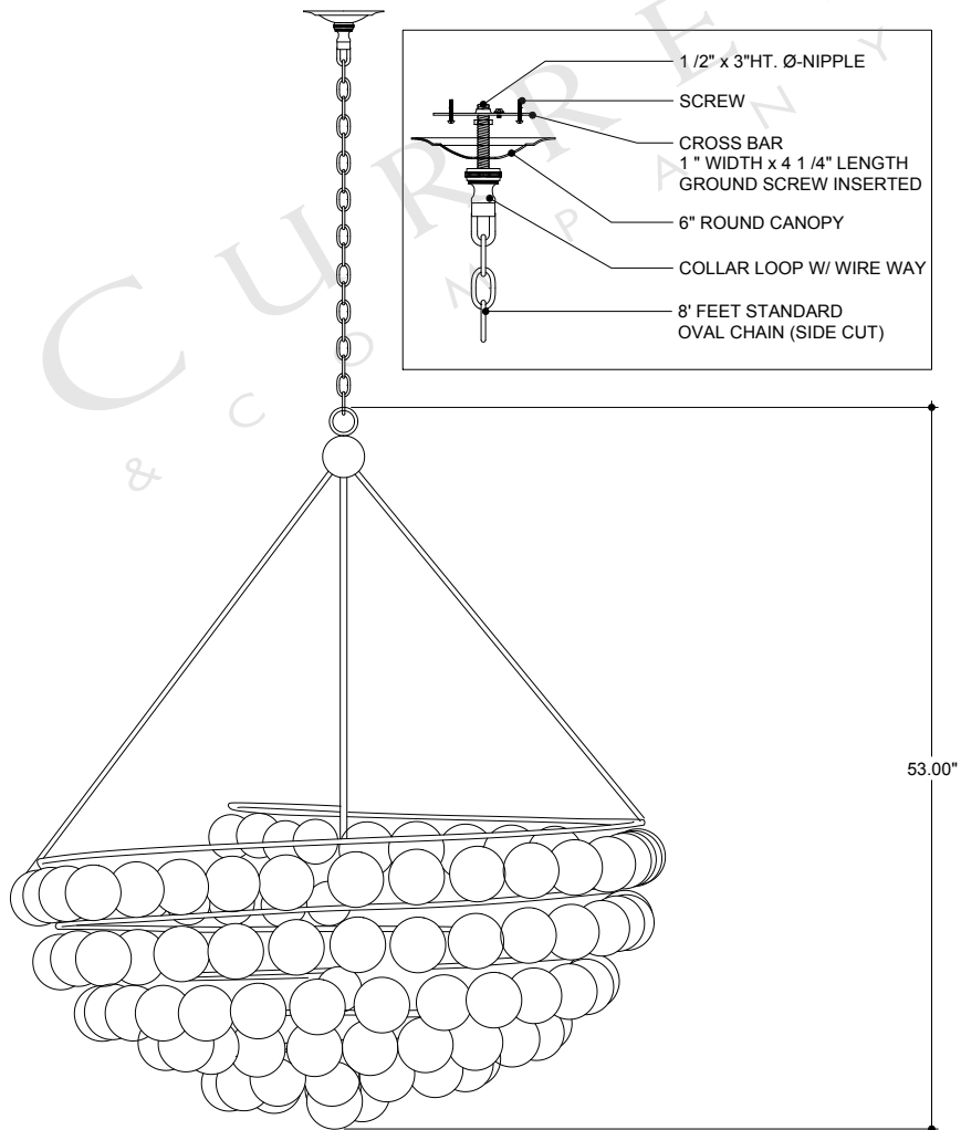
FRONT VIEW
