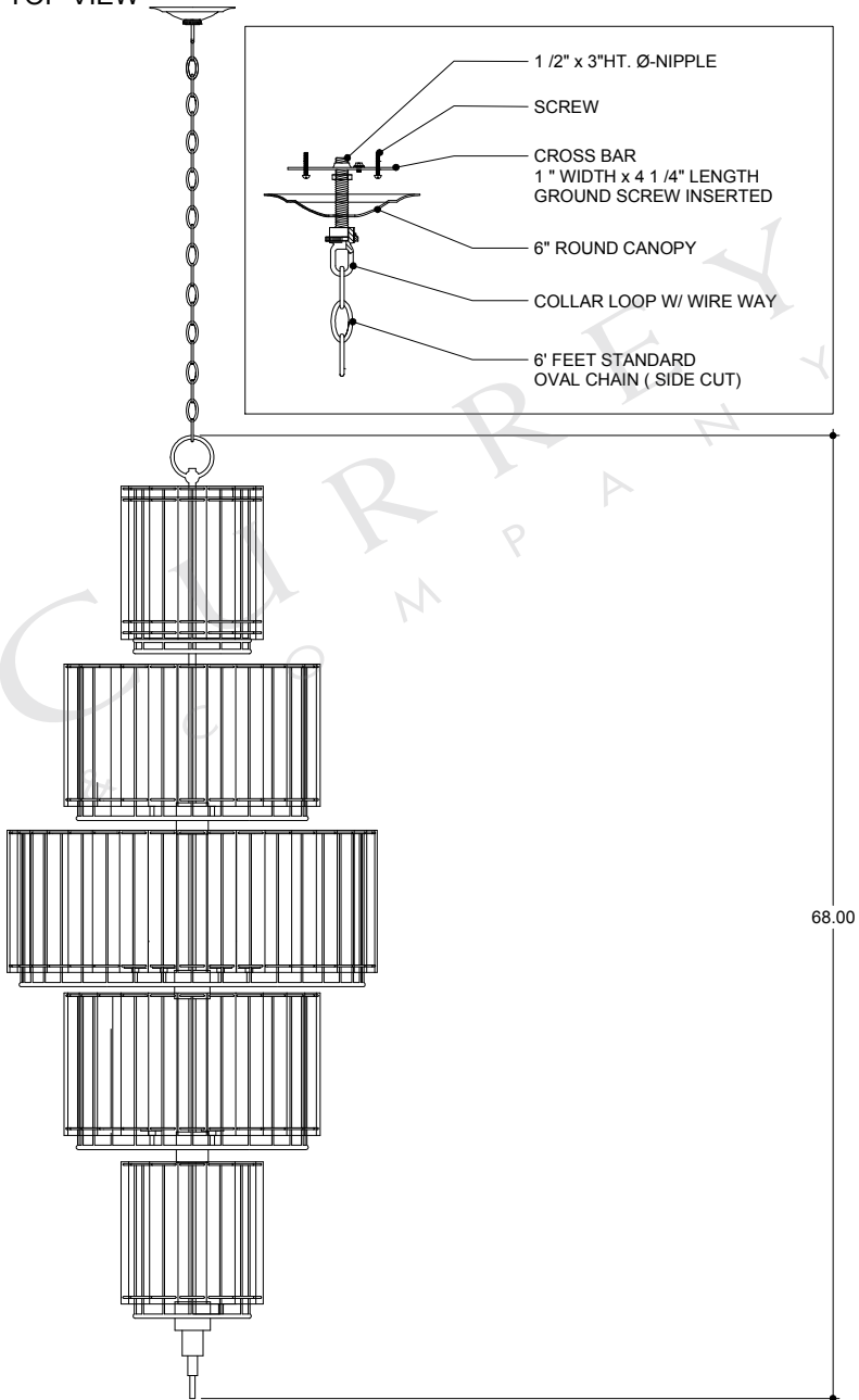
FRONT VIEW
