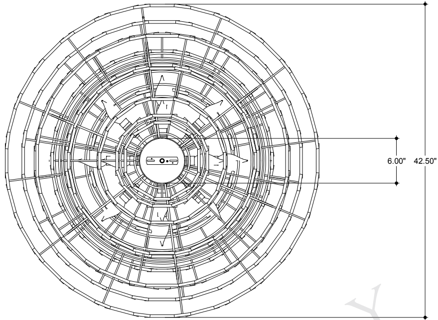
TOP VIEW
