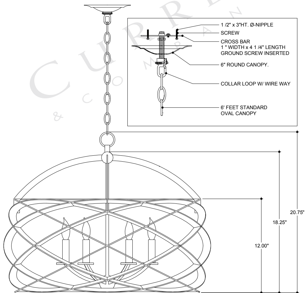
FRONT VIEW
